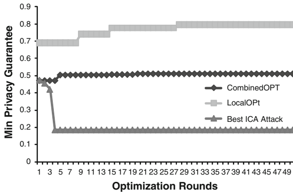
Fig. 17 Optimization of perturbation for votes data
