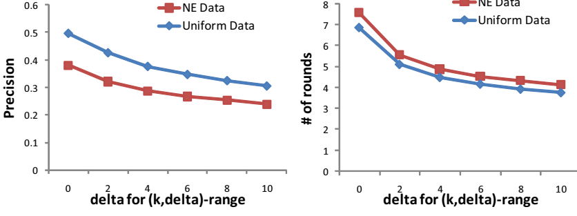
Fig. 10. Performance and result precision for different \delta setting of the (k, \delta) -range algorithm for 2-dimensional data.
