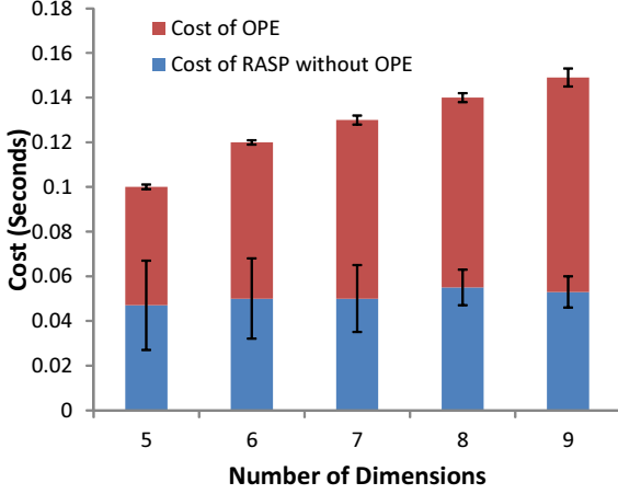
Fig. 6. The cost distribution of the full RASP scheme. Data: Adult (20K records, 5-9 dimensions)
