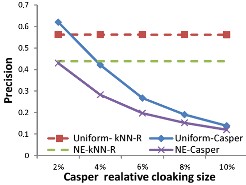
Fig. 12. The impact of cloaking-box size on precision for Casper for the NE data.
