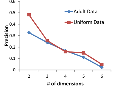
Fig. 11. Precision reduction with more dimension.
